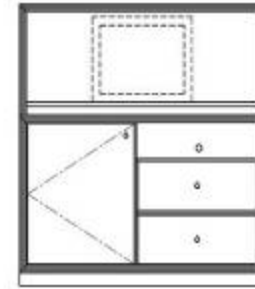
PL-104 Fridge Chest D24xW64xH40 inches
