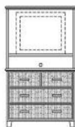
TRP-110 Chest with LCD Hutch D20xW38xH60 inches
